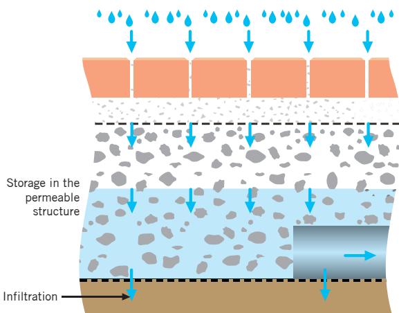
Figure 21: Attenuation and infiltration storage volume.
