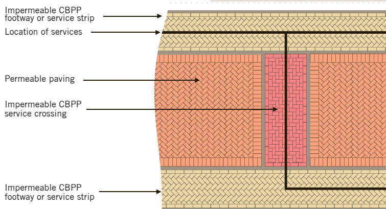
Figure 13: Plan and cross section of a typical service crossing.
