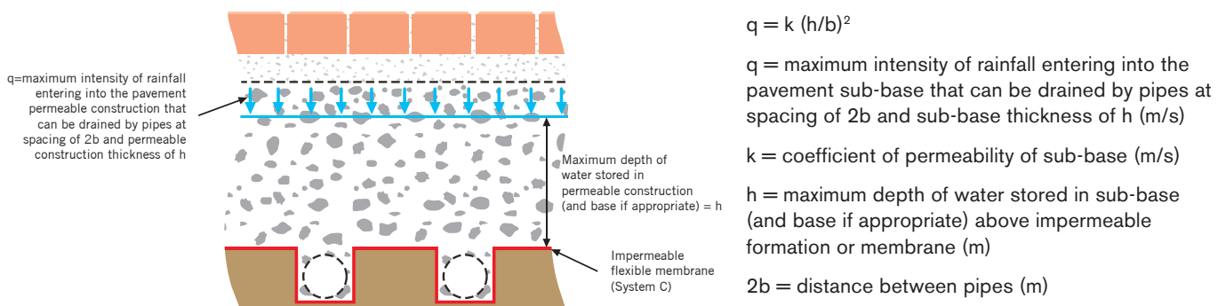
Figure 27: Estimating outfall pipe spacing
