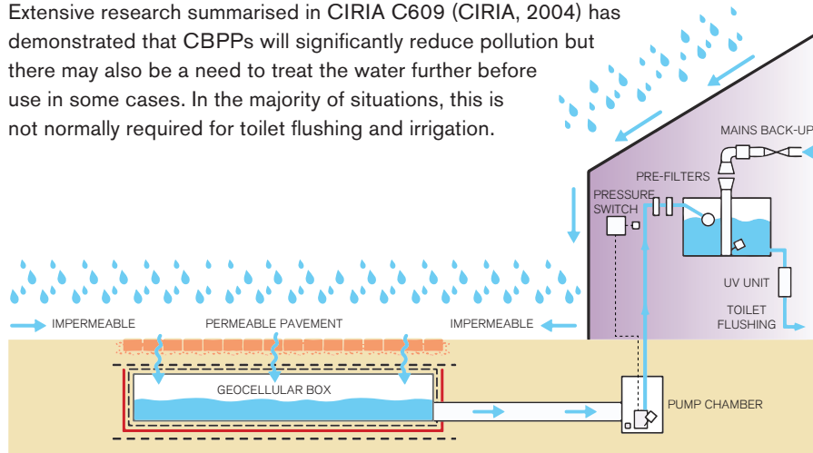
Figure 14: Example of a rainwater harvesting system
