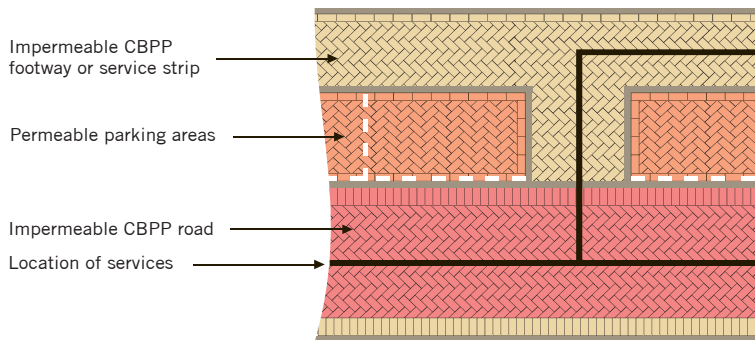
Figure 12: Plan of a layout with services in road and footway.
