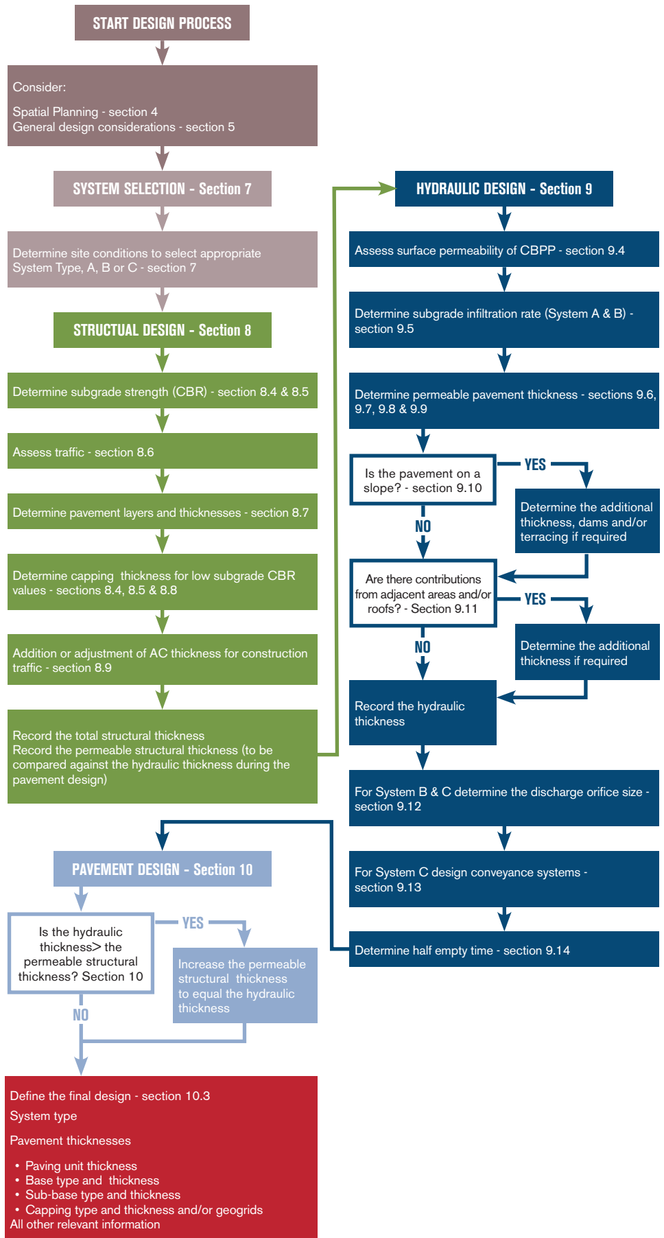
Figure 16: Engineering design procedure for CBPP
