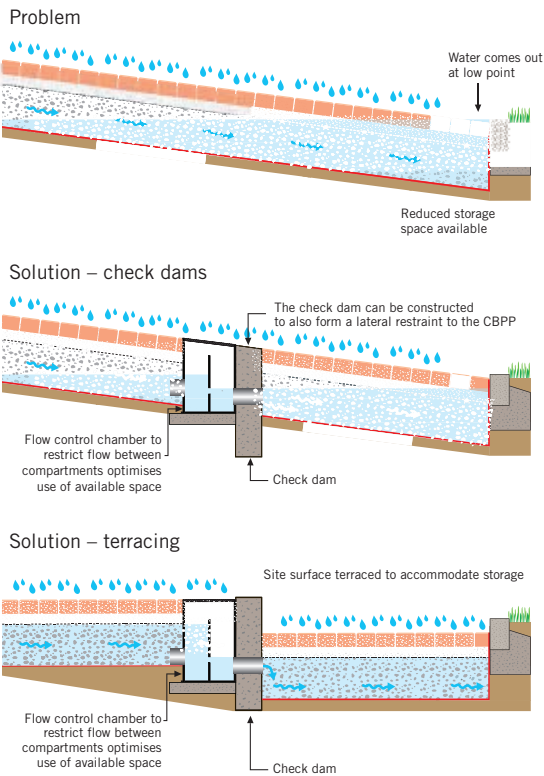
Figure 10: Managing CBPPs on sloping sites.
