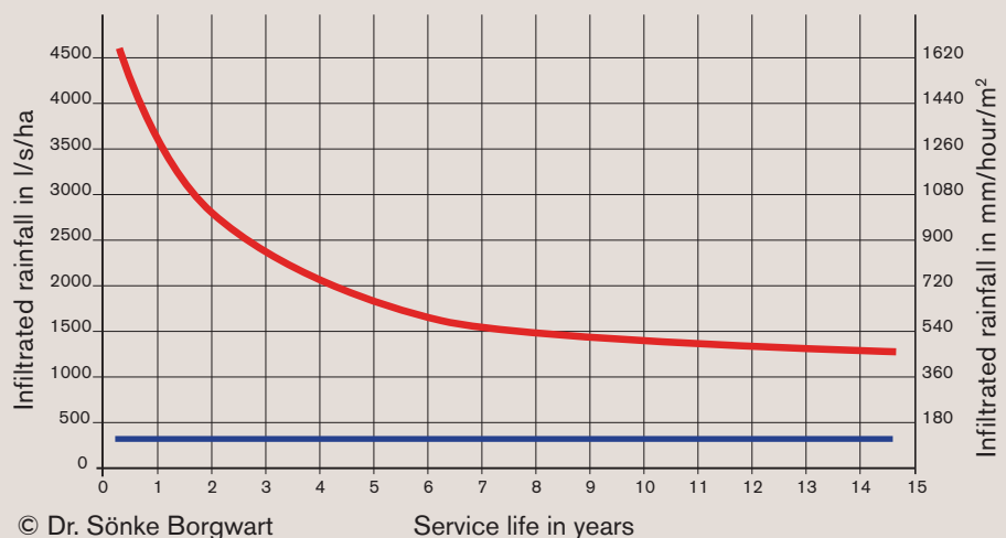
Figure 20: Typical reduction of surface infiltration rate over time.
